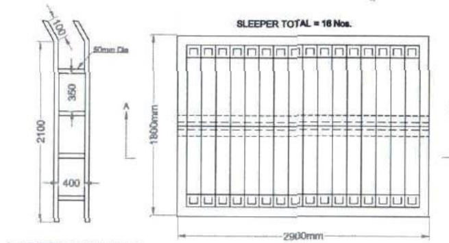
LADDER DETAILS
